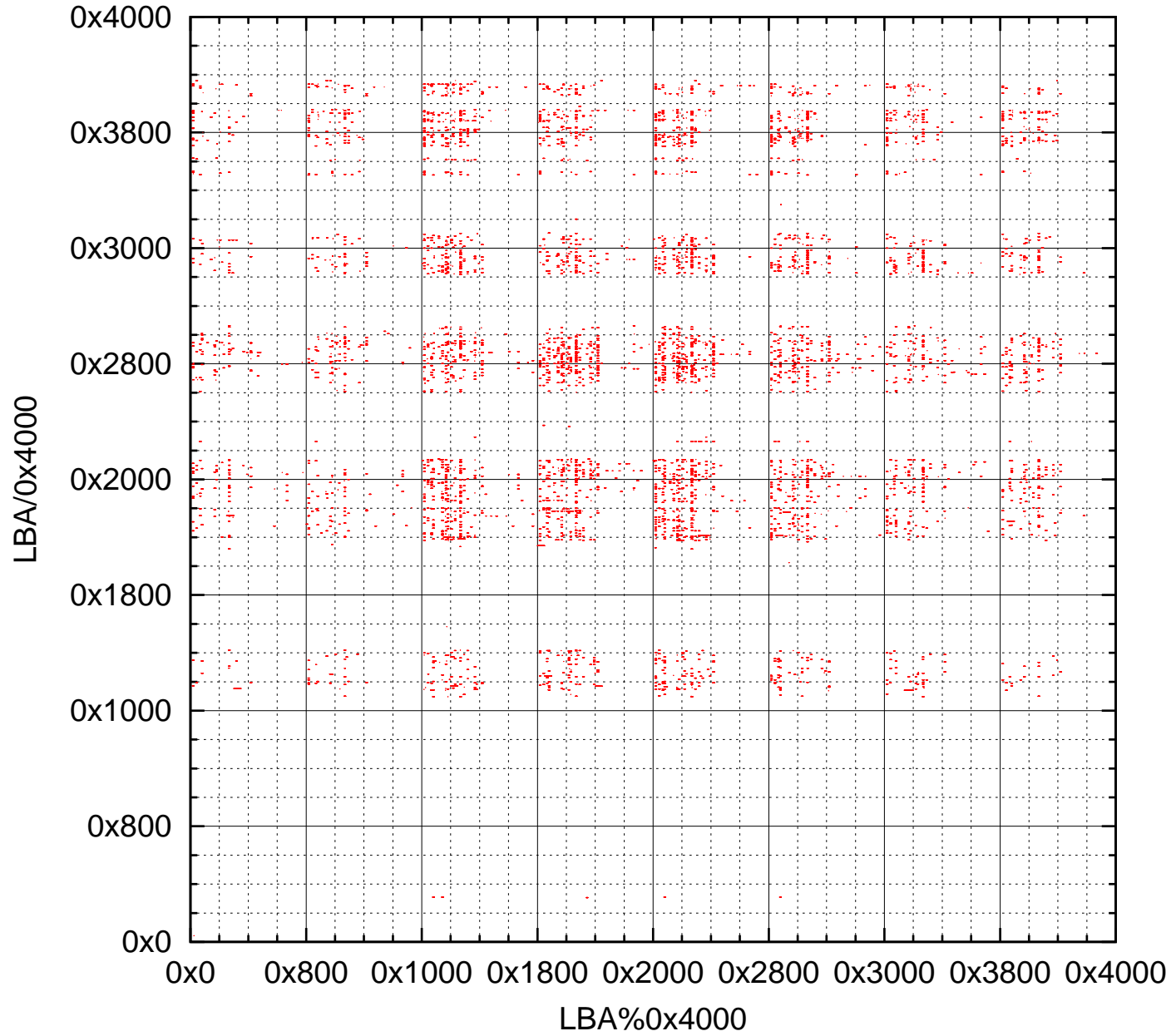
SAMSUNG 470 128Gbyte (MZ5PA128HMCD-0AA00) bad blocks
